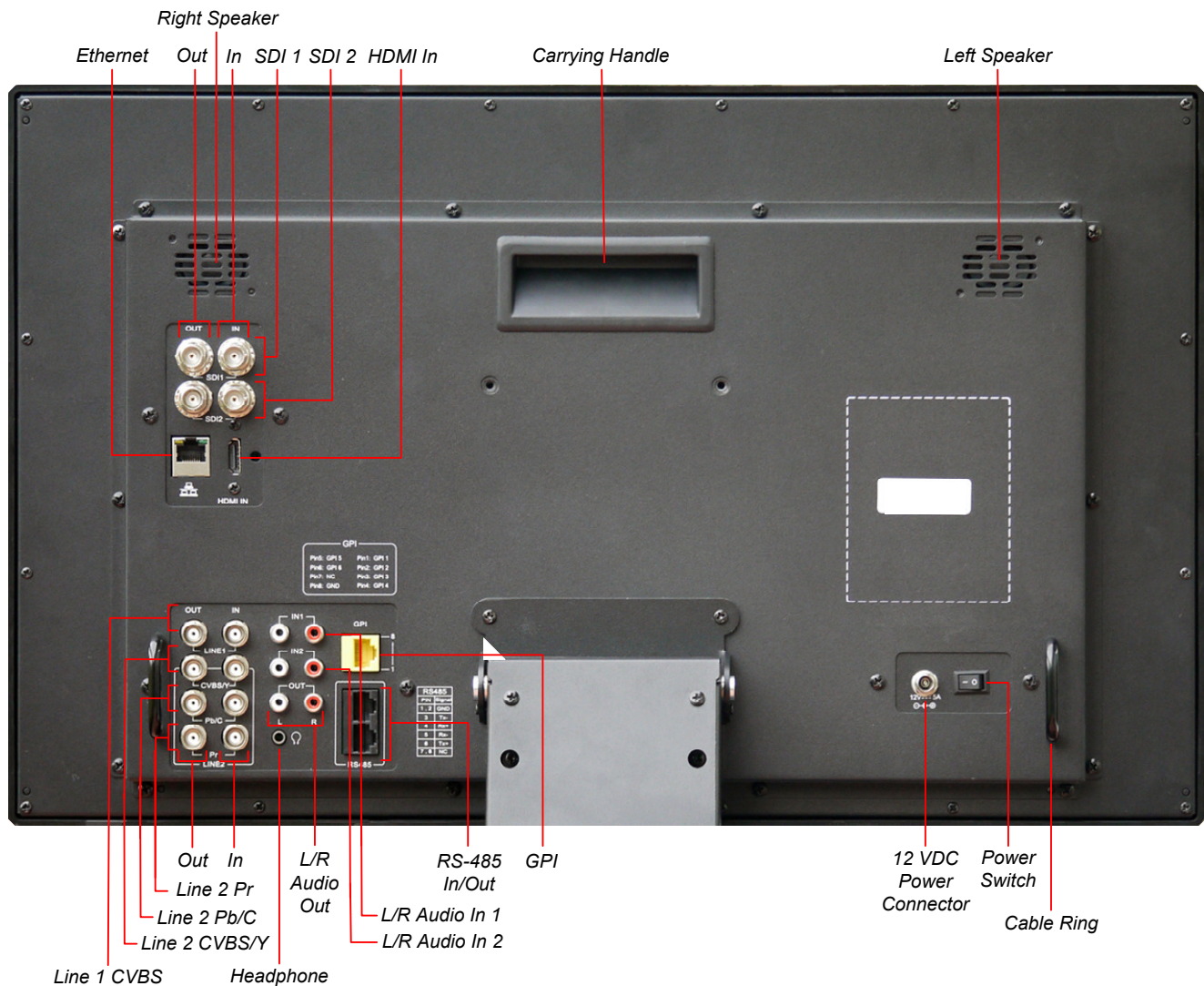
Figure 2-3: Rear Panel Layout
