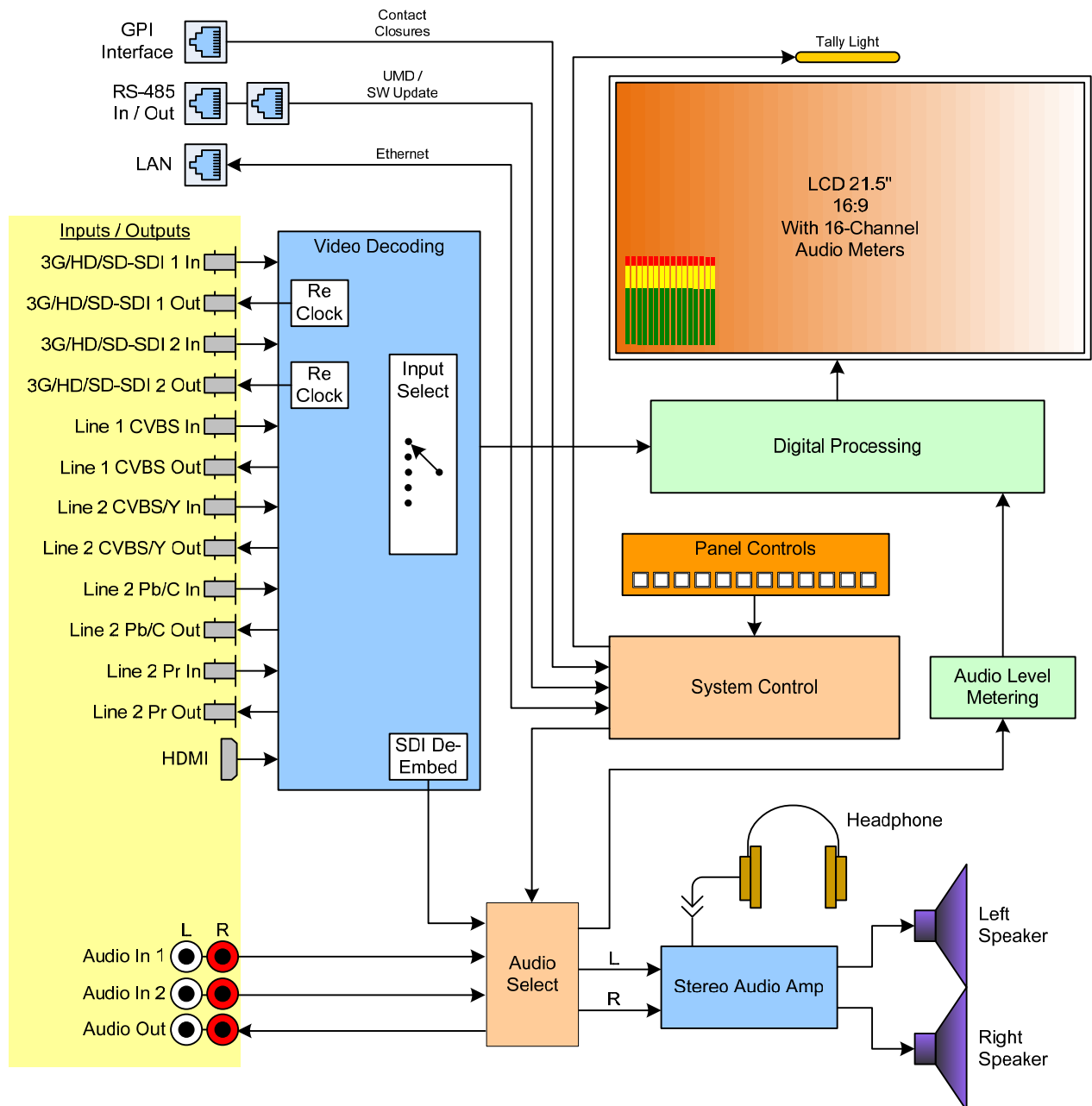
Figure 3-1: HDM-215-3G Series Block Diagram
