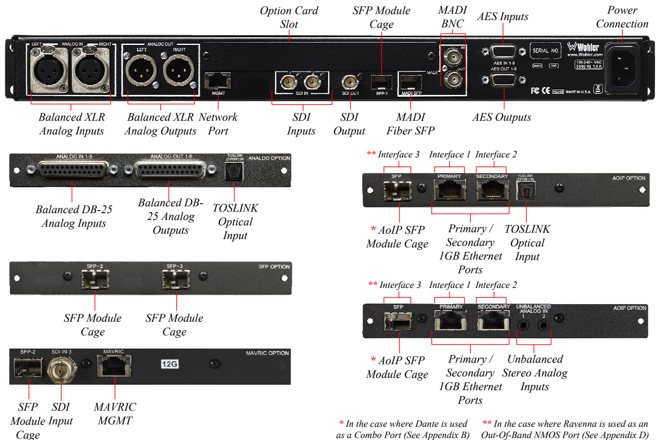
Figure 2-2: iAM-AUDIO-1 PLUS Rear Panel & Option Cards
