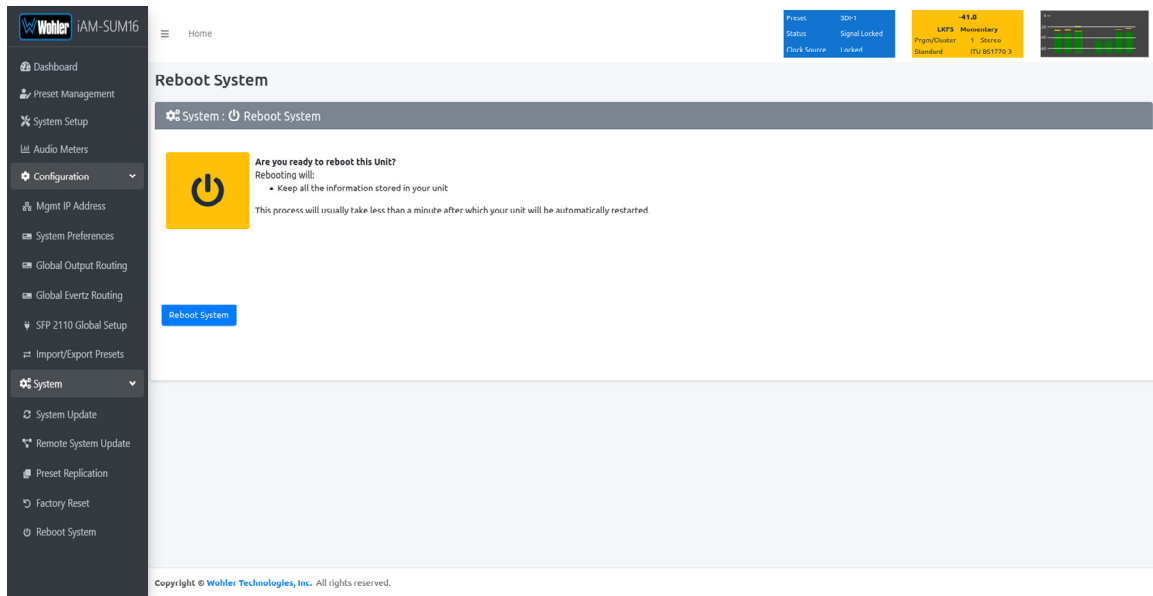
Figure 4-37: Reboot System
