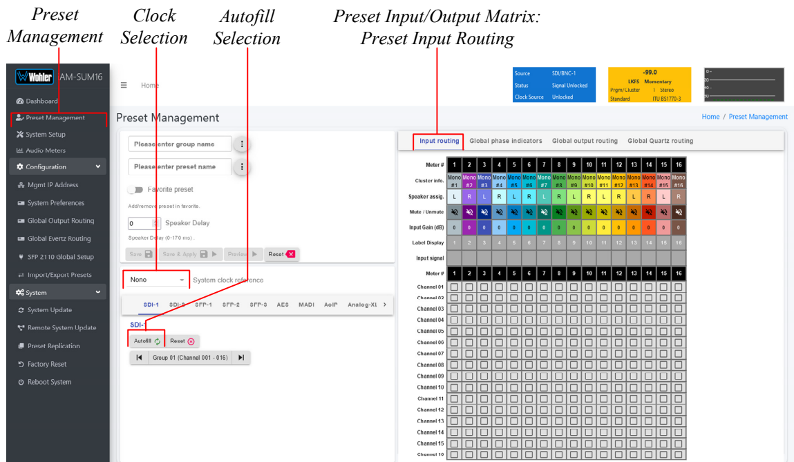
Figure 4-17: Configure Presets
