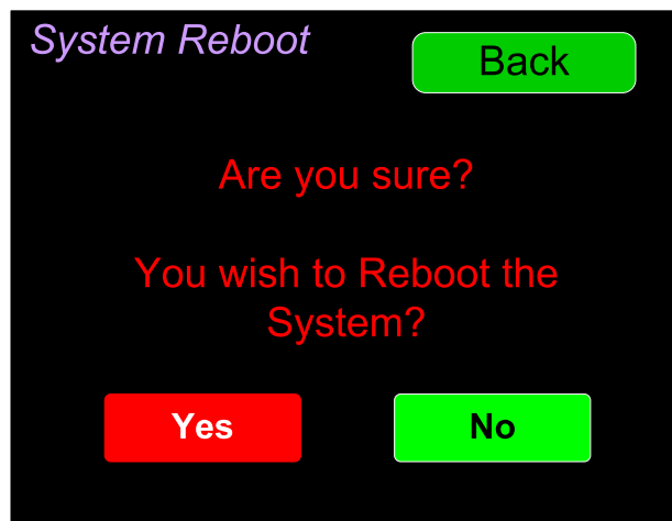
Figure 2-33: System Reboot
