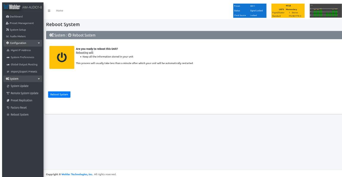
Figure 4-32: Reboot System
