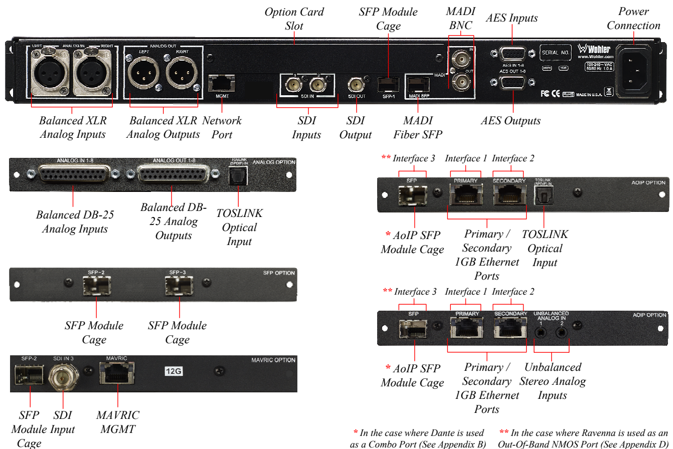
Figure 2-2: iAM1-8 Rear Panel & Option Cards
