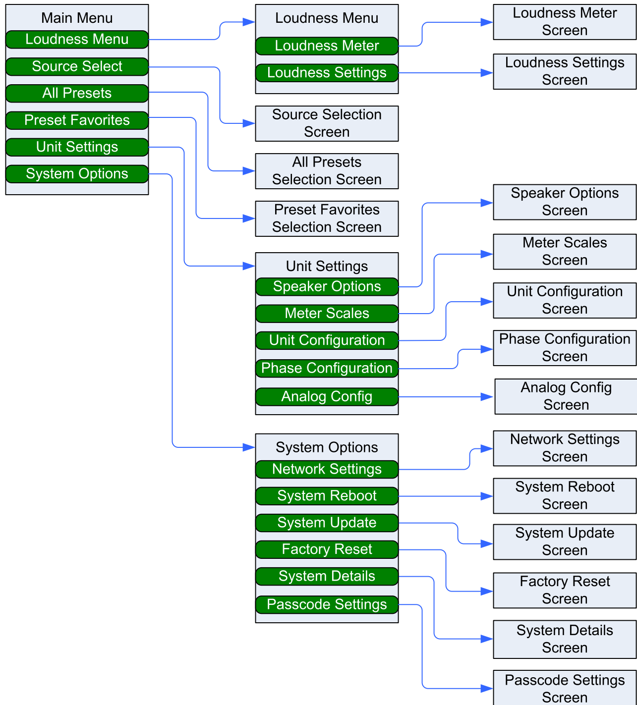
Figure 2-10: Menu Tree
