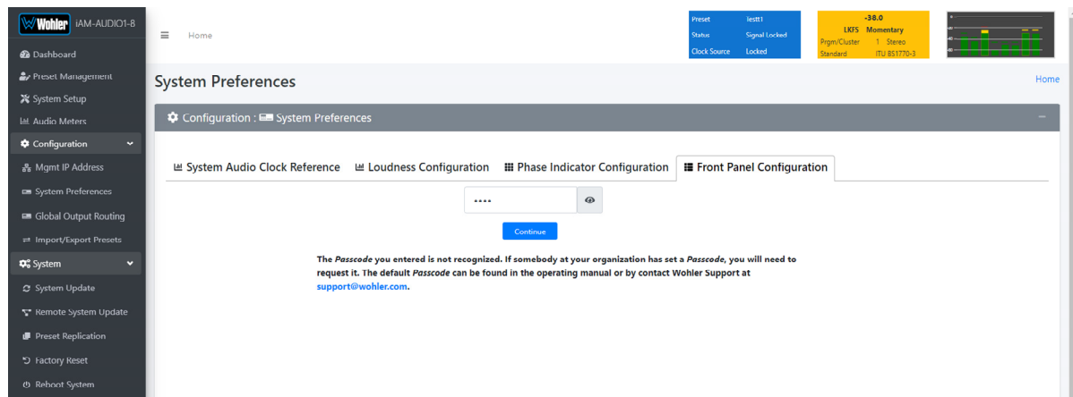
Figure 4-12: Unrecognized Passcode
