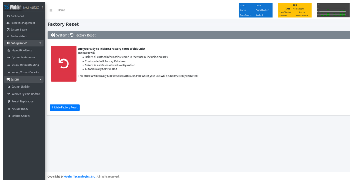
Figure 4–31: Factory Reset
