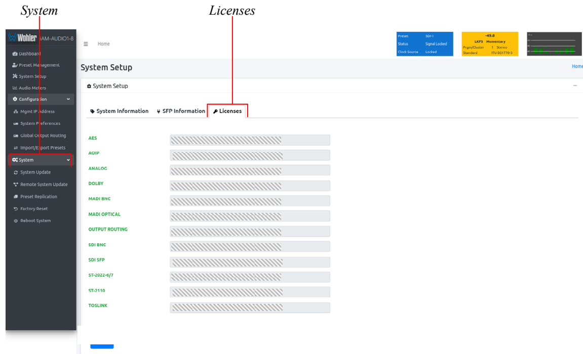
Figure 4-30: Licenses Tab
