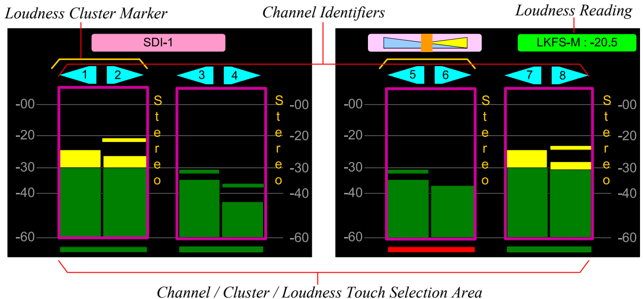
Figure 2-8: Audio Level Meter Screens
