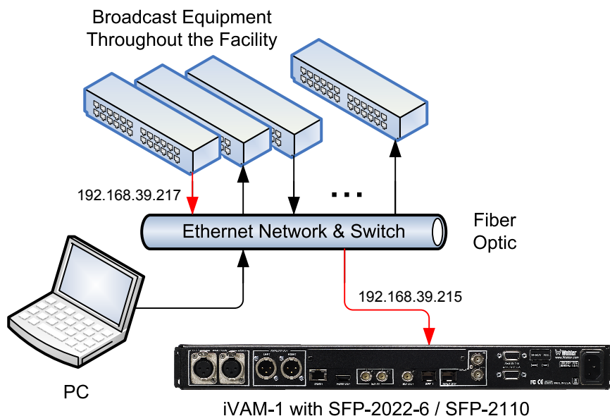
Figure 2-8: SFP-2022-6 and SFP2110 Network Diagram
