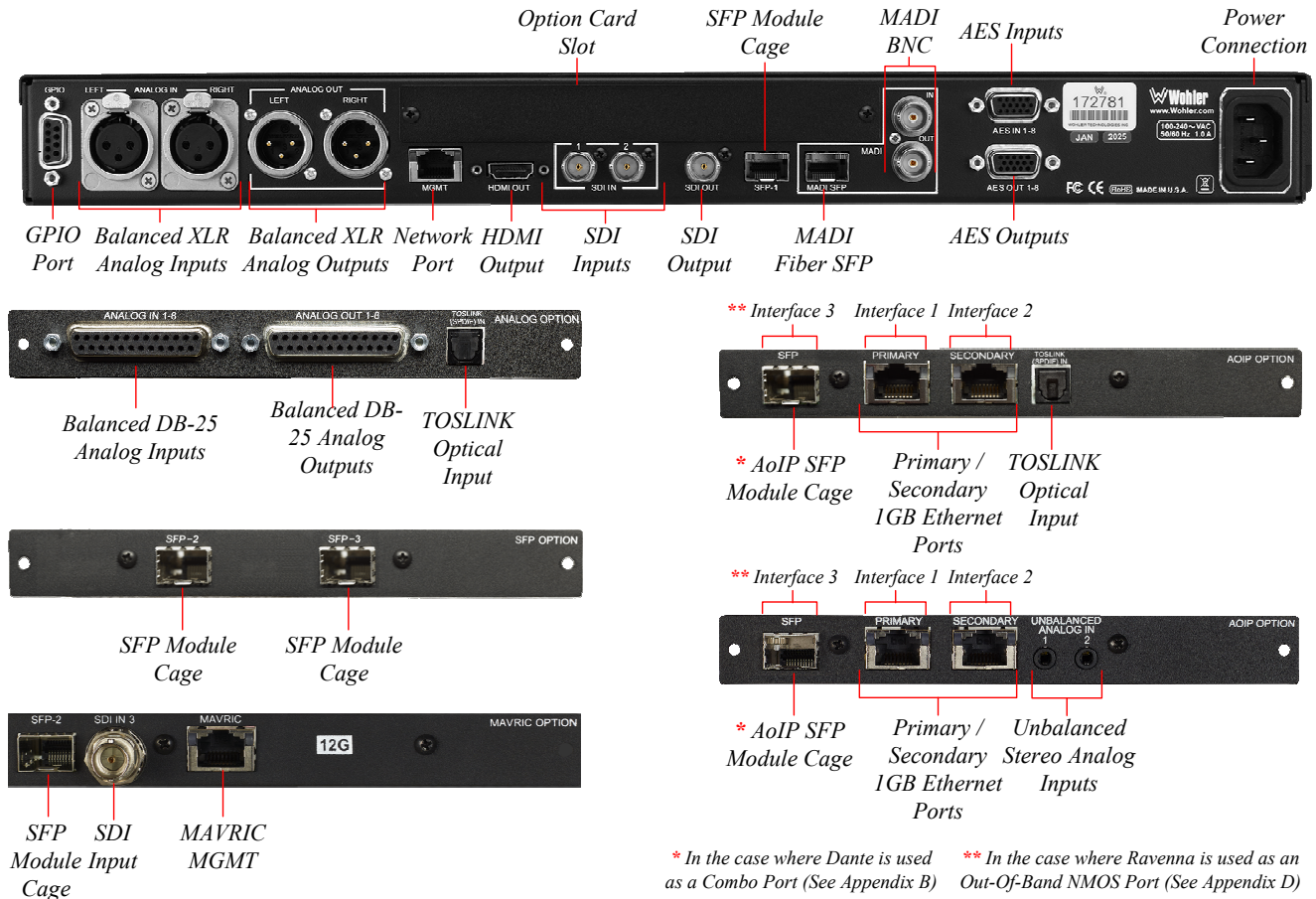
Figure 2-2: iVAM1-1-G Rear Panel and Option Cards
