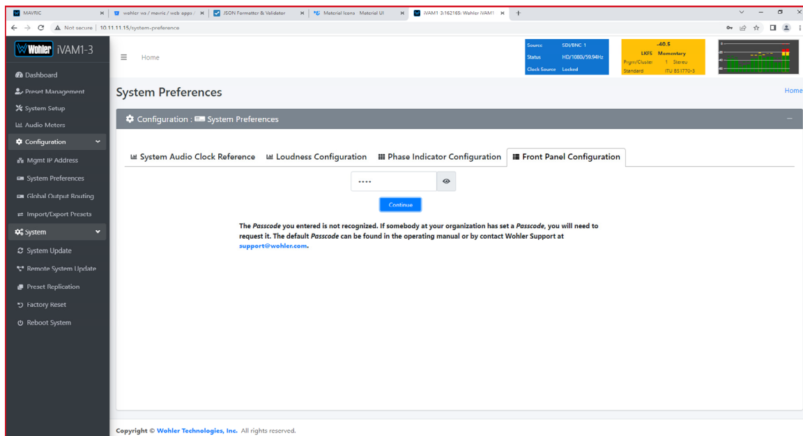
Figure 4-12: Unrecognized Passcode
