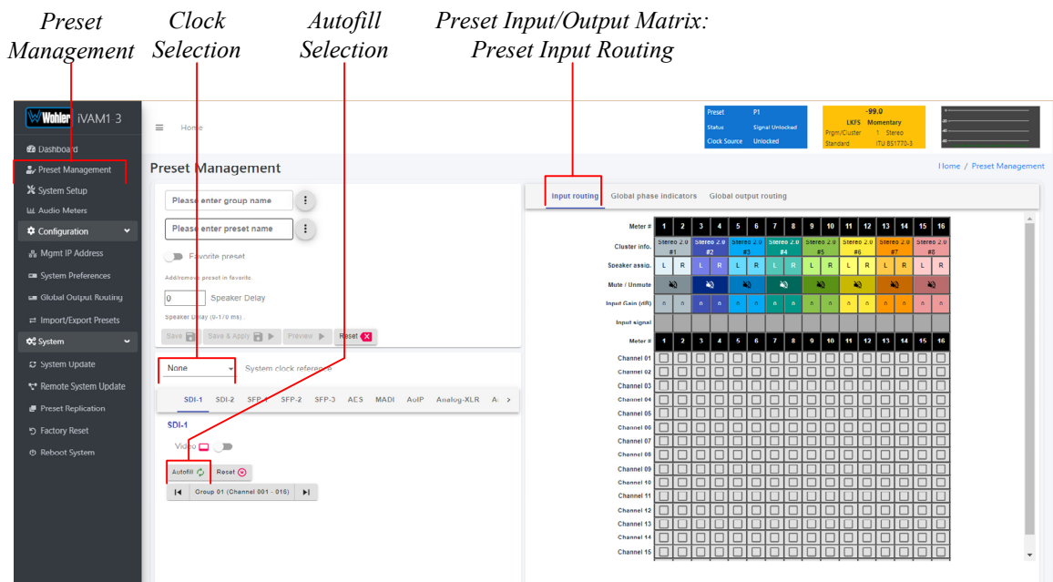
Figure 4-17: Configure Presets
