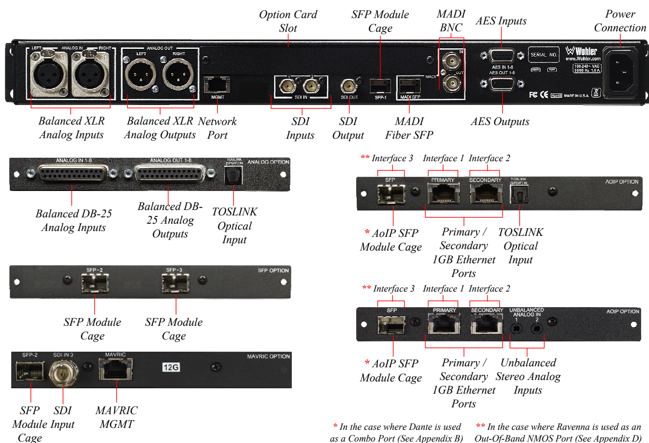
Figure 2-2: iVAM1-3 Rear Panel & Option Cards
