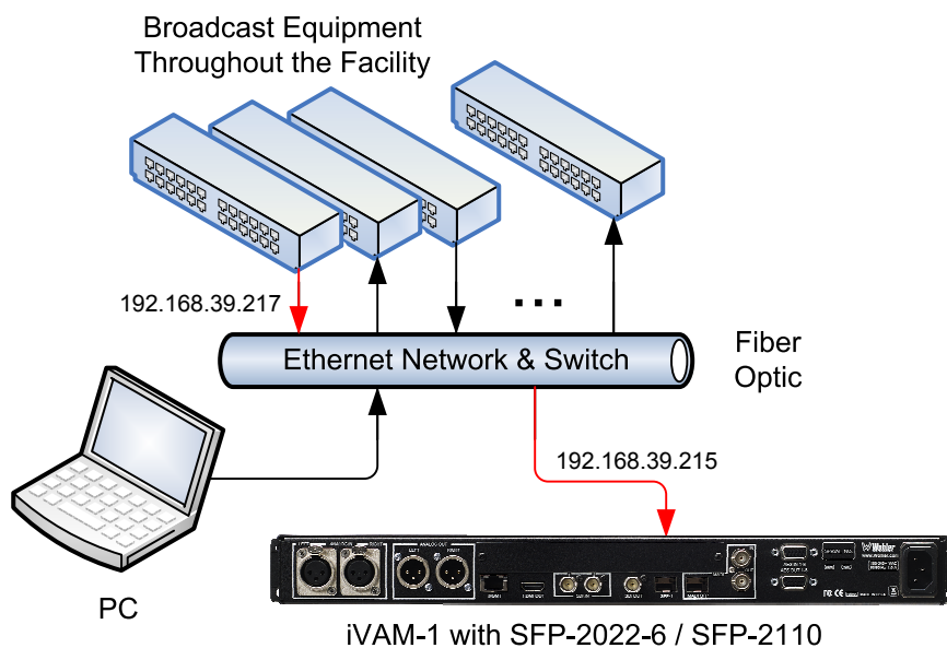
Figure 2-7: SFP-2022-6 and SFP2110 Network Diagram
