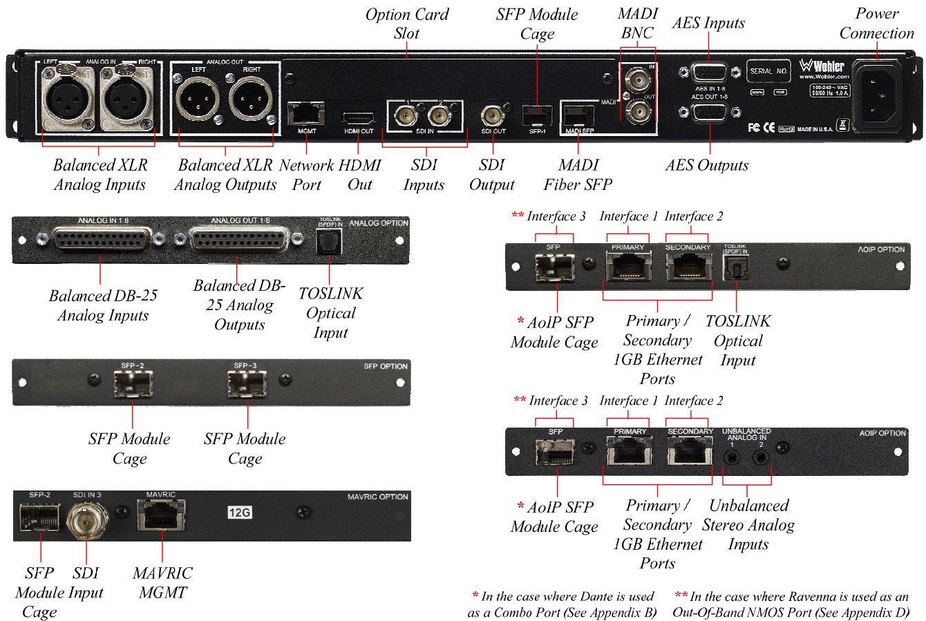
Figure 2-2: /VAM1-SUM16-12G Rear Panel & Option Cards
