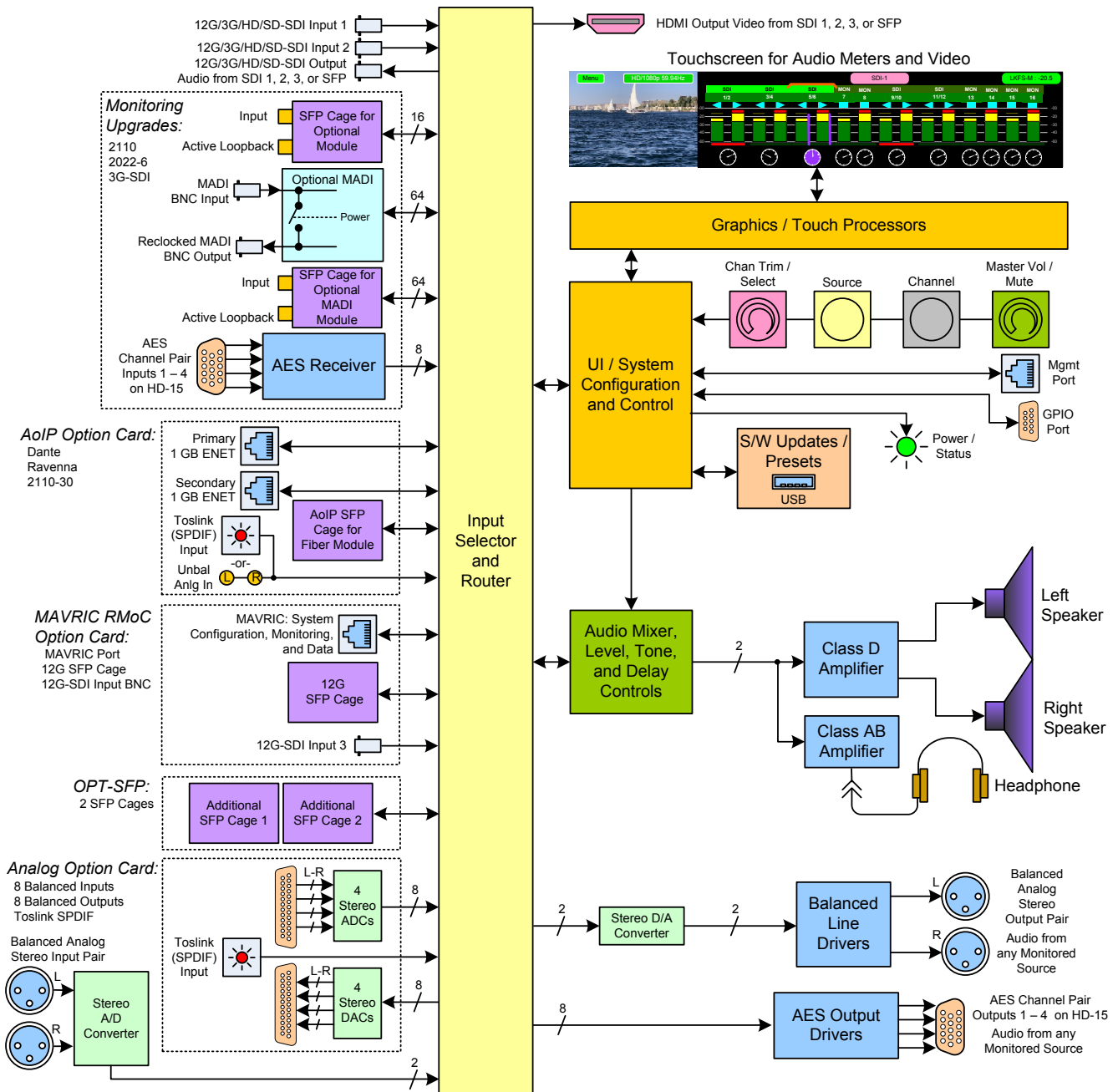
Figure 3-1: /VAM1-SUM16-12G Block Diagram
