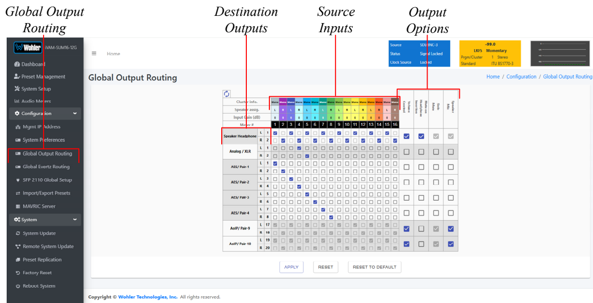
Figure 4-20: Global Output Routing Option
