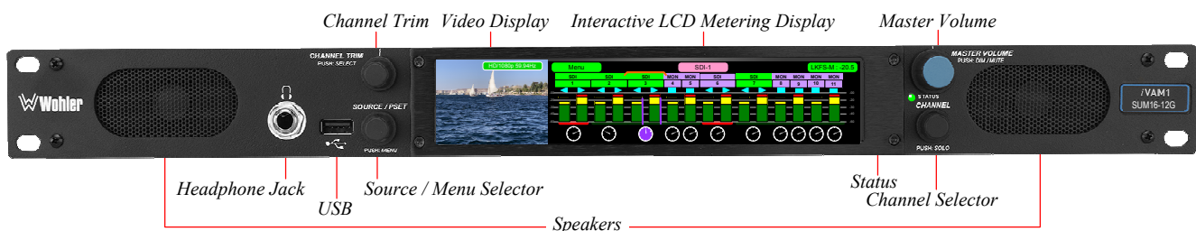
Figure 2-1: /VAM1-SUM16-12G Front Panel
