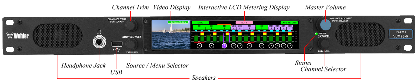
Figure 2-1: /VAM1-SUM16-G Front Panel
