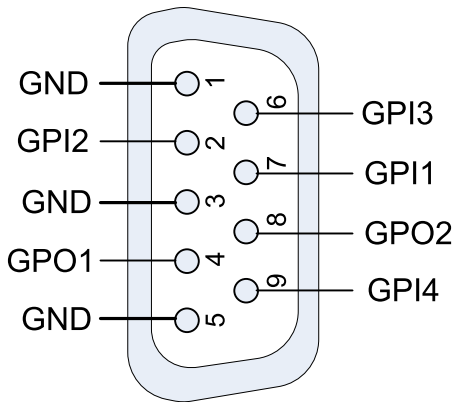
Figure 2-7 – GPIO Port Pinout
