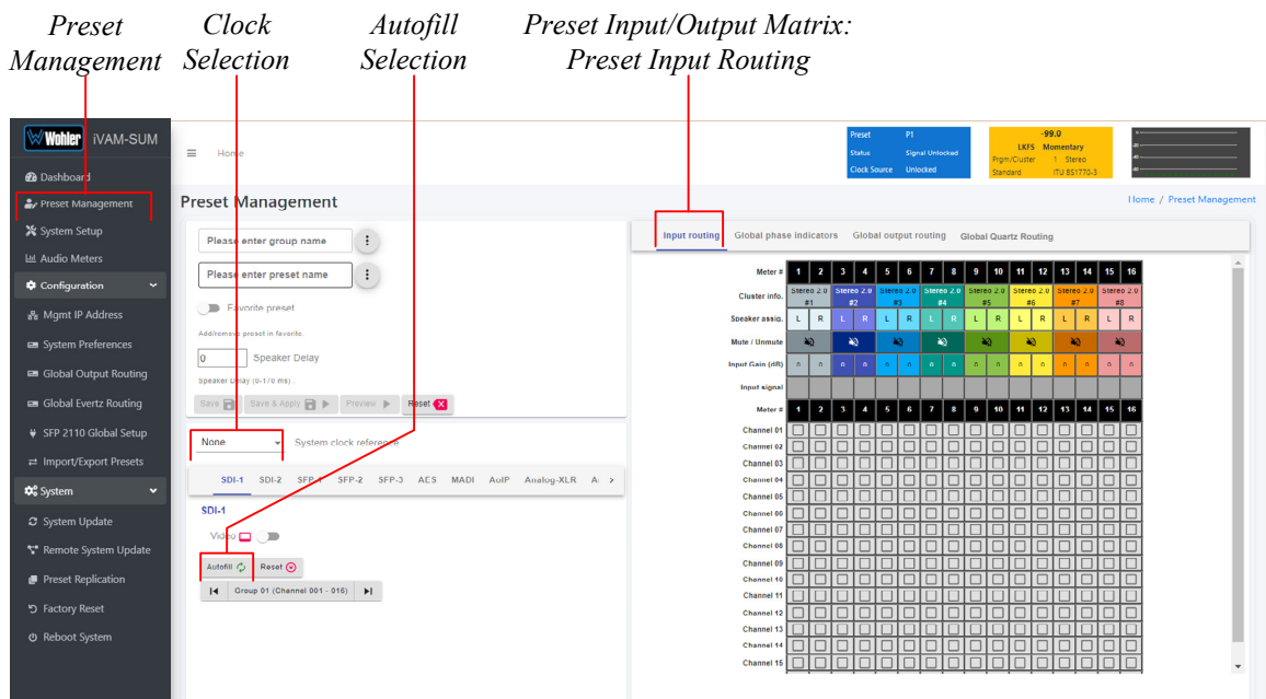
Figure 4-18: Configure Presets
