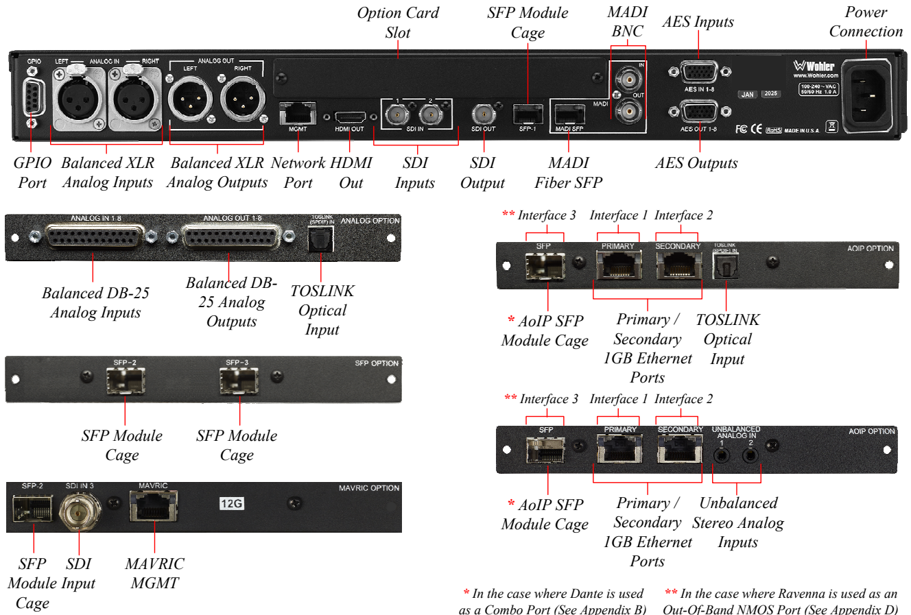
Figure 2-2: /VAM1-SUM16-G Rear Panel & Option Cards
