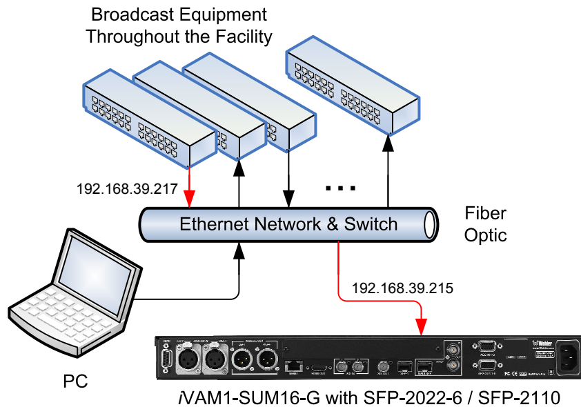
Figure 2-8: SFP-2022-6 and SFP2110 Network Diagram
