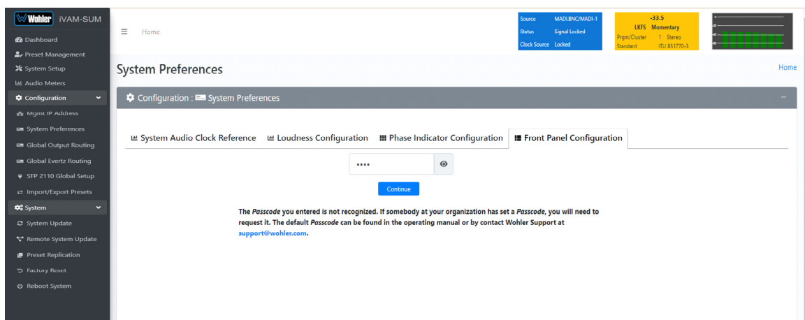
Figure 4-13: Unrecognized Passcode
