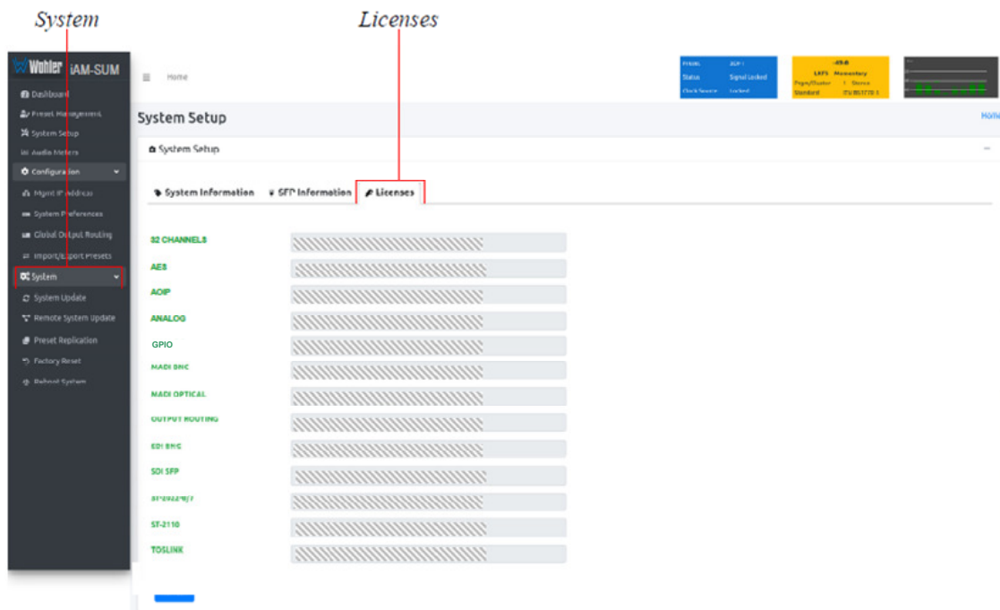
Figure 4-34: Licenses Tab
