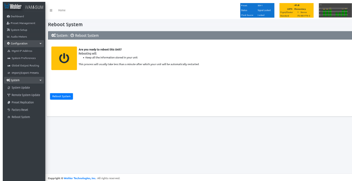
Figure 4-36: Reboot System
