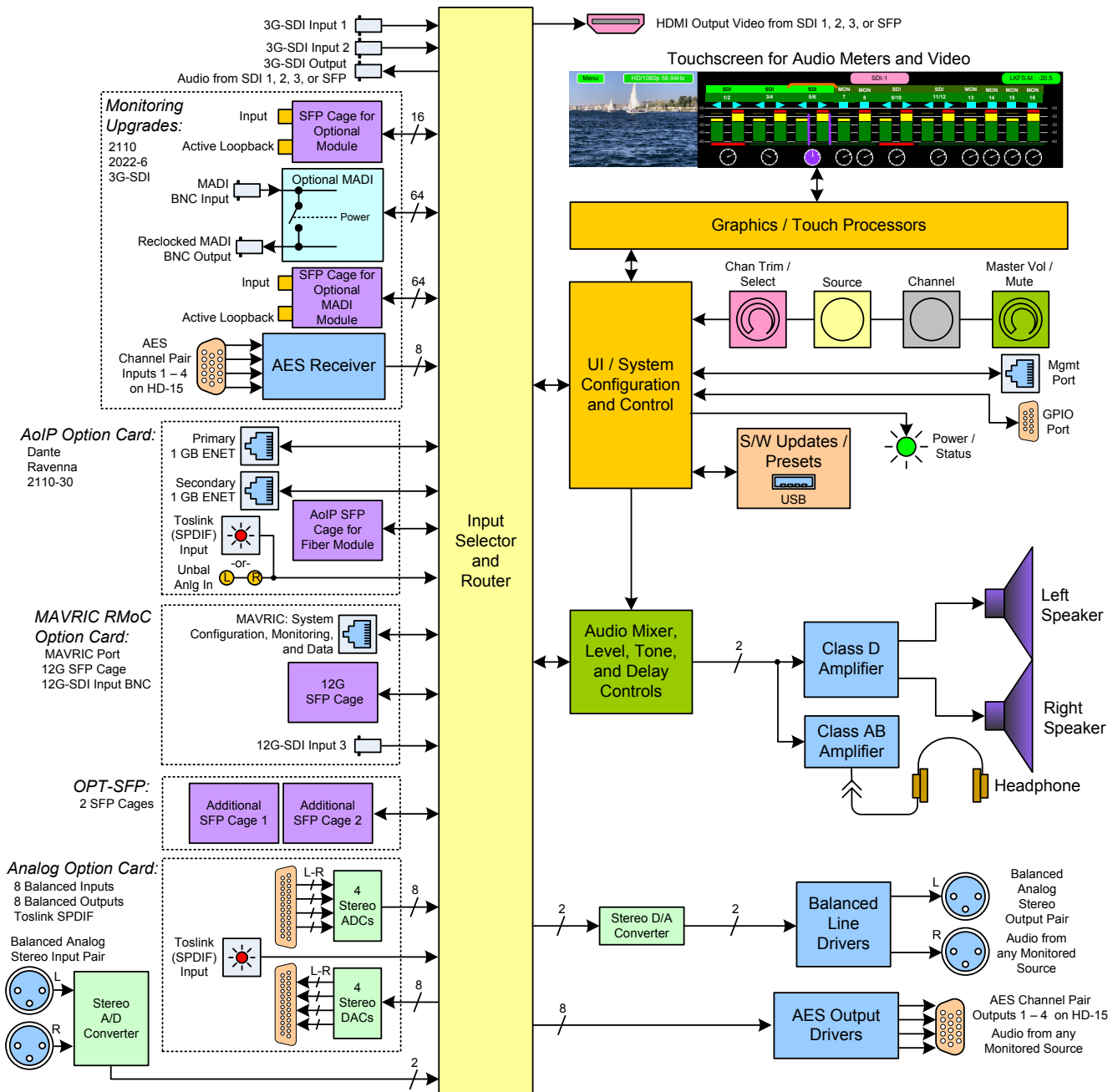
Figure 3-1: /VAM1-SUM16-G Block Diagram
