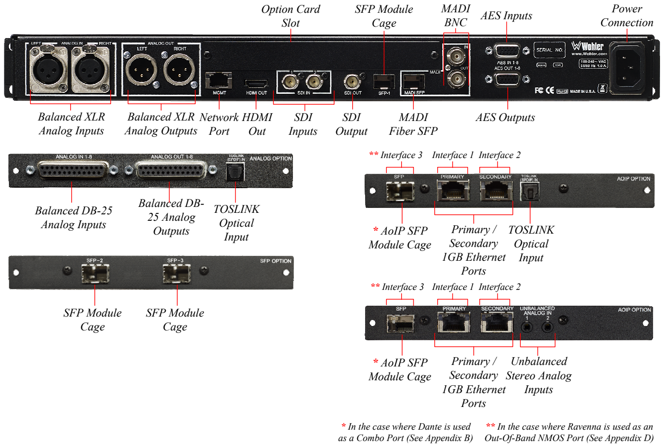
Figure 2-2: iVAM1-SUM Rear Panel & Option Cards
