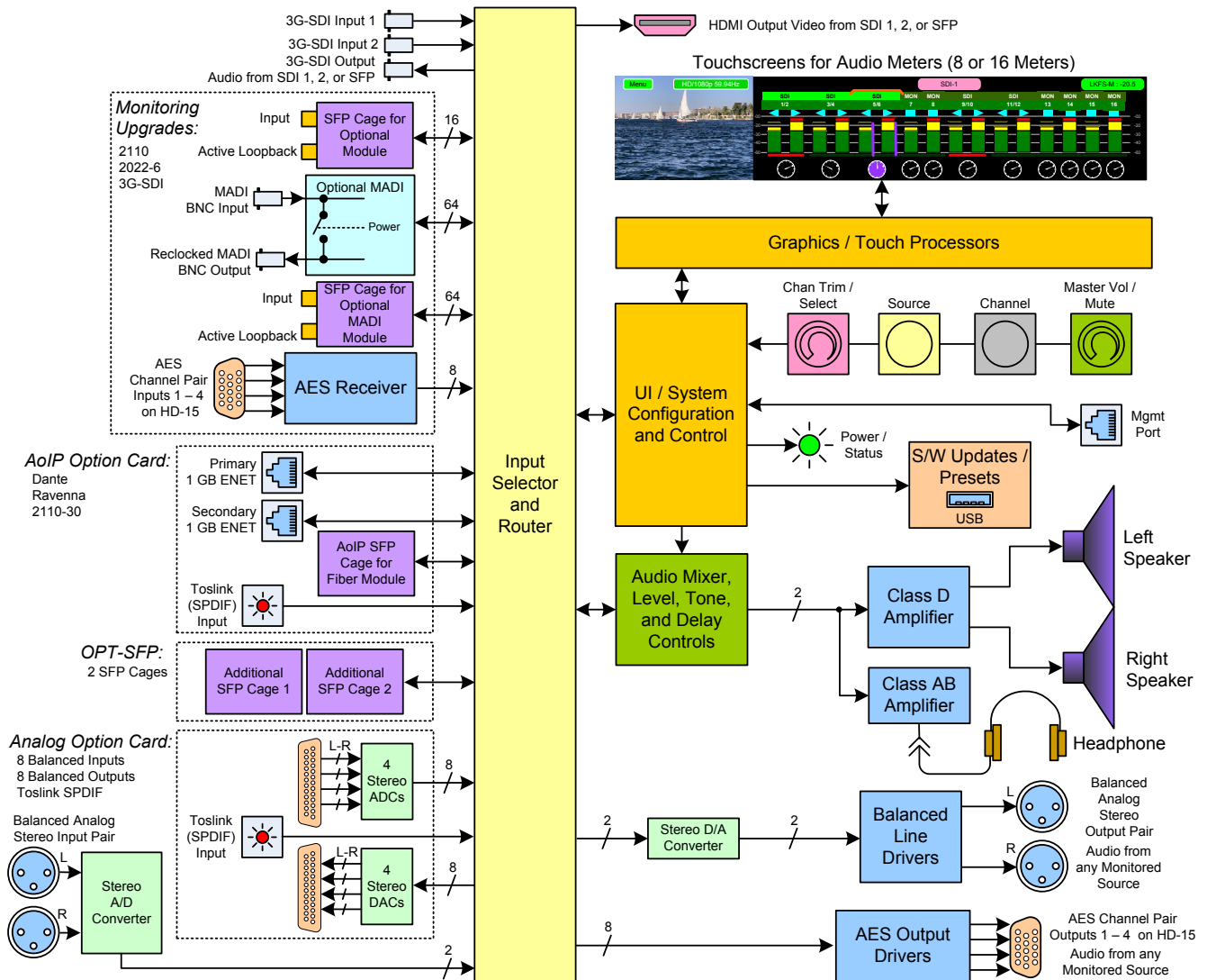
Figure 3–1: iVAM1-SUM Block Diagram
