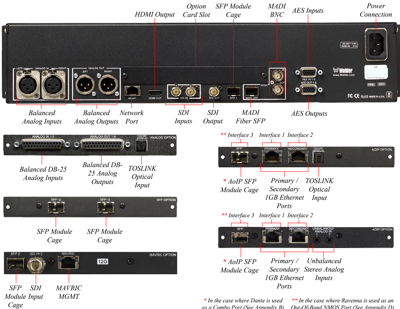
Figure 2-2: iVAM2-12G Rear Panel & Option Cards
