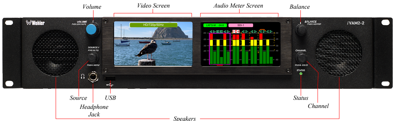
Figure 2-1: iVAM2-2 Front Panel
