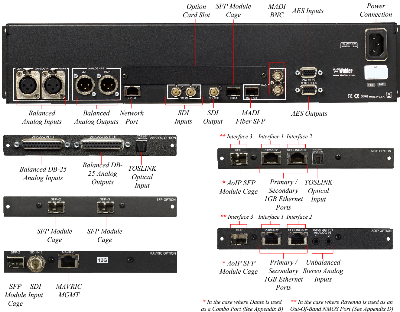
Figure 2-2: iVAM2-2 Rear Panel & Option Cards
