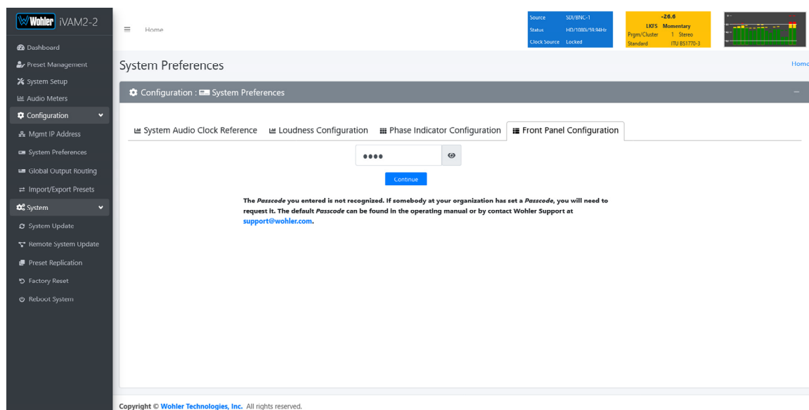
Figure 4-12: Unrecognized Passcode
