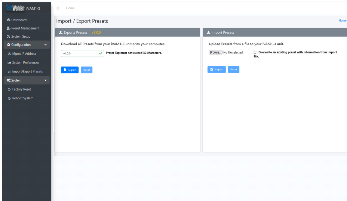
Figure 4–25: Database Export
