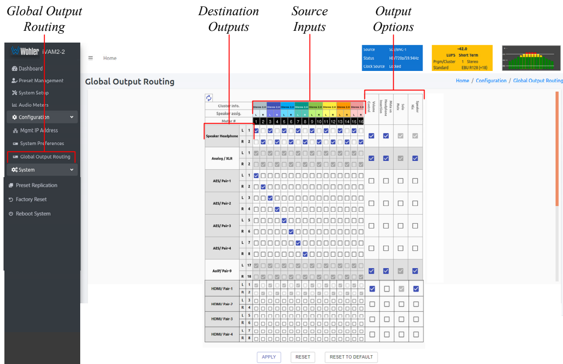
Figure 4-22: Global Output Routing Option
