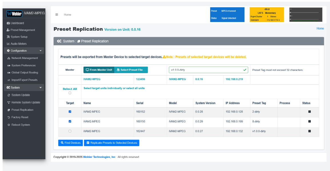
Figure 4-21: Preset Replication Target Selection Screen
