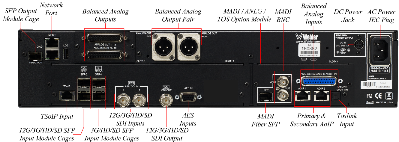
Figure 2-2: iVAM2-MPEG Rear Panel Layout
