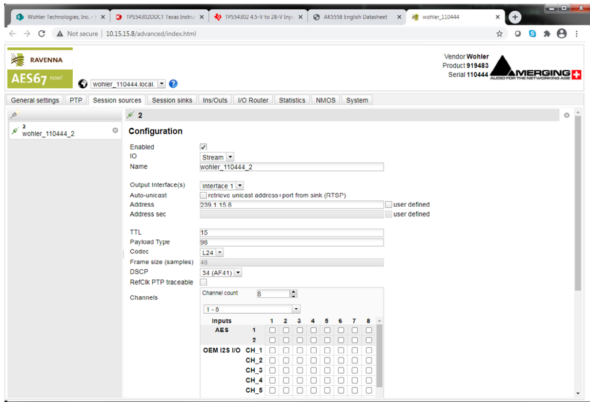
Figure D-11: Session Sources Tab
