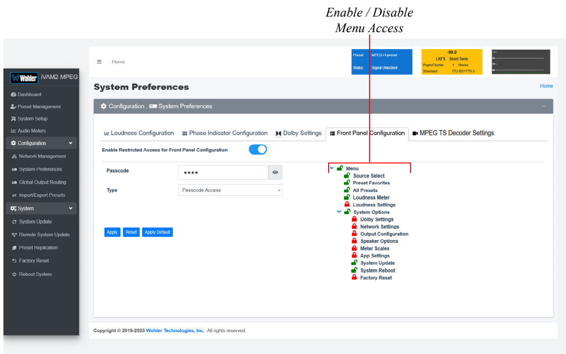
Figure 4-34: Front Panel Configuration Tab
