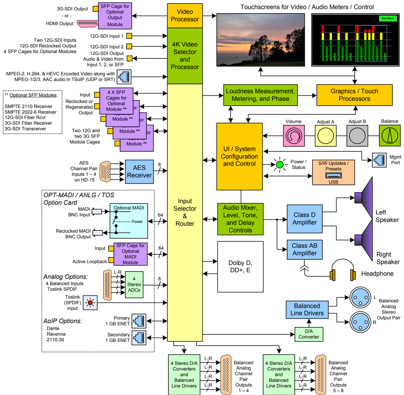
Figure 3-1: iVAM2-MPEG Block Diagram
