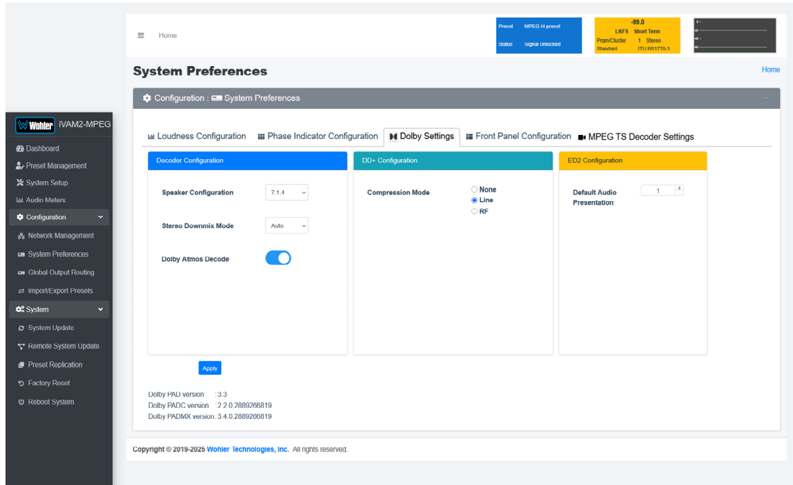
Figure 4-31: Dolby Settings Tab
