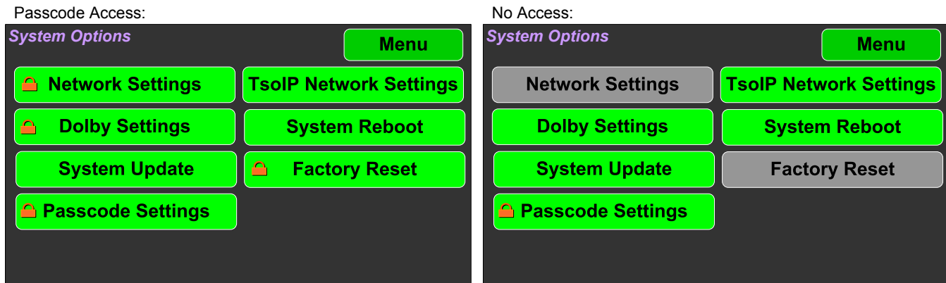
Figure 2-46: Examples of Menu Protection
